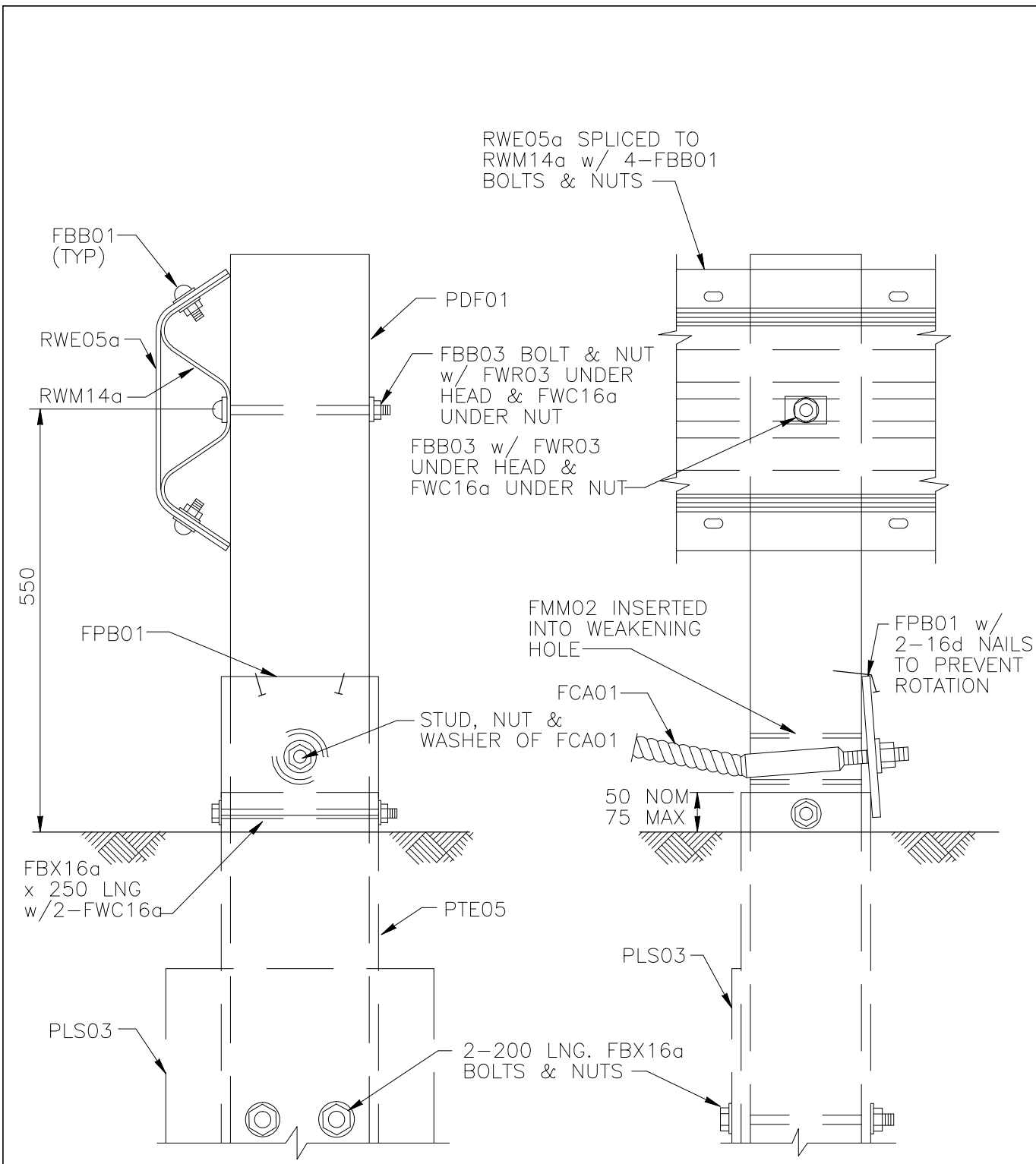
DETAIL E: POST 1 ASSEMBLY-SEW03a
