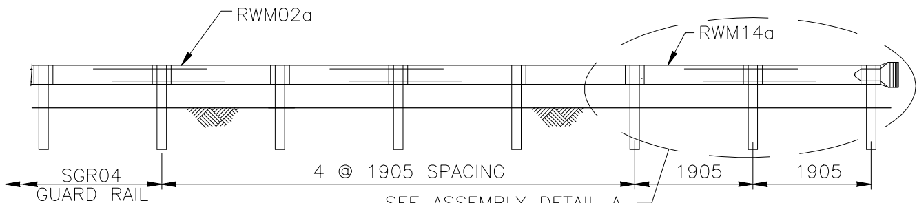
PLAN
