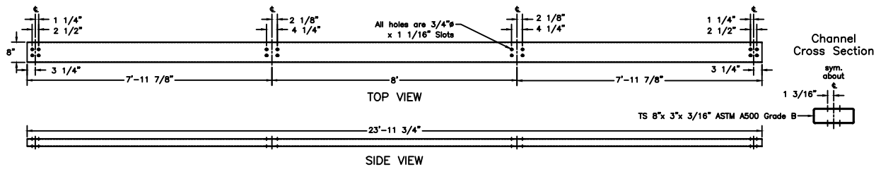
Upper Tube Rail, Type 1
