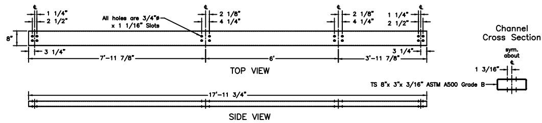
Upper Tube Rail, Type 2
