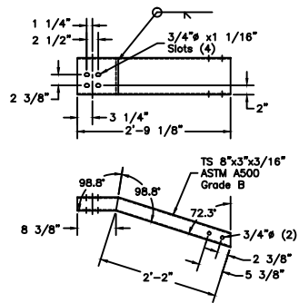
Tube Transition Rail #2
