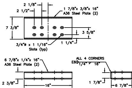
Transition Splice Tube
