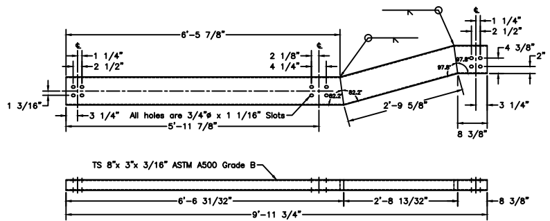
Tube Transition Rail #1
