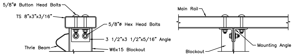
Tube Rail Connection
