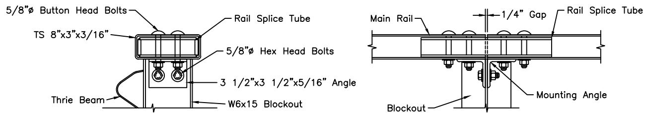
Tube Rail Splice
