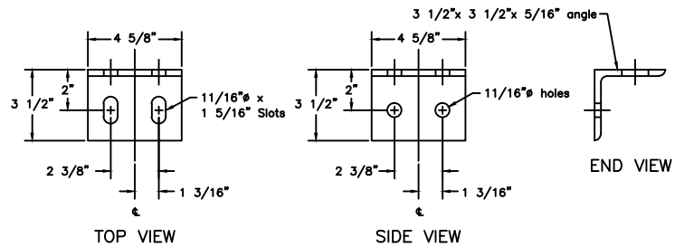
Mounting Angle
