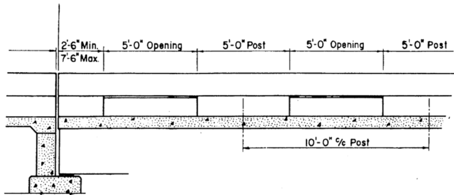
ROADWAY ELEVATION OF RAIL
