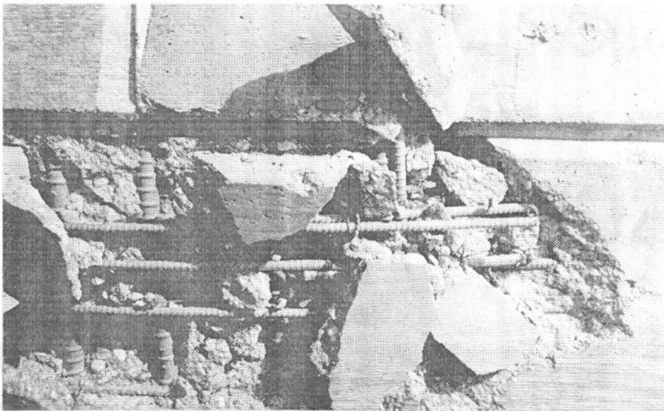
Figure 25. Post No. 5 damage at splice and deck cracking
