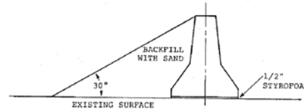
FIGURE 60. CONCRETE BARRIER INSTALLATION SUPPORT.
