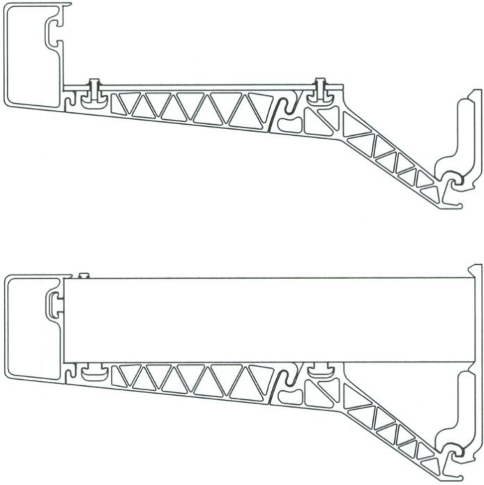
SECTION AT POST
