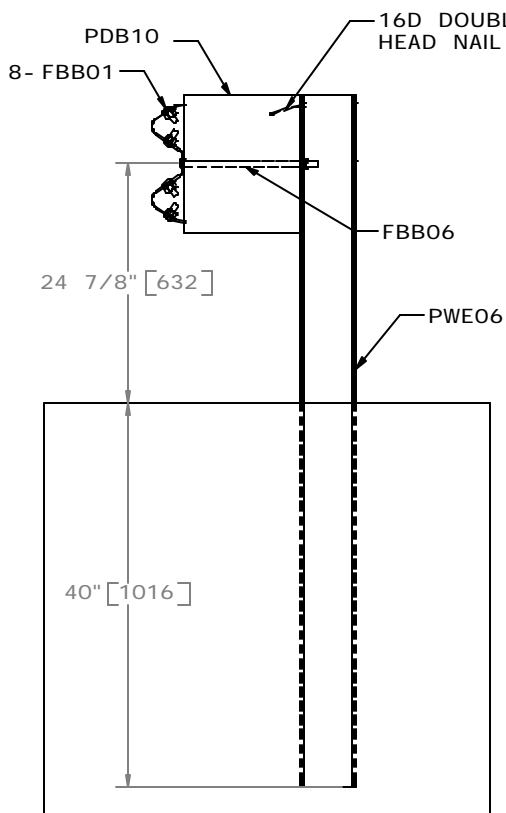
SGR22a Section A- A
